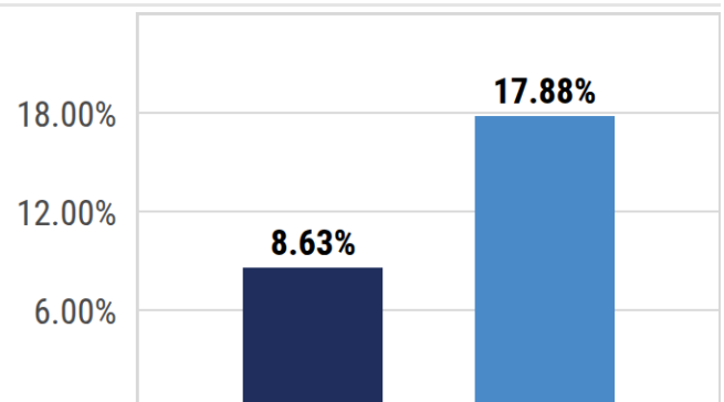
Tariff Drawdown & Recovery (01/01/2025 - 12/31/2025)
